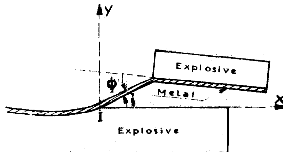
Fig 4 - Experimental arrangement
